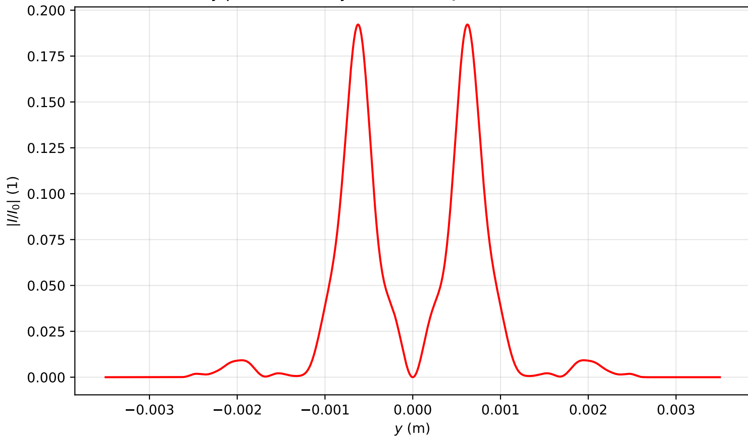
Intensity profile I(x=0, y, z=2.070)/I_0 , P_{in}=5.0P_{cr} , artificial time
